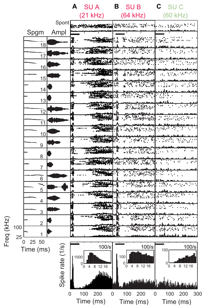
Figure 5. Example SU Responses to Natural Pup Calls
