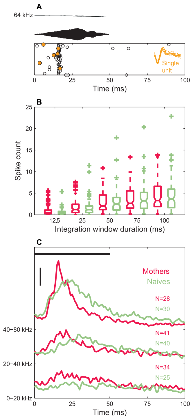
Figure 1. Responses from Mothers and Naïve Females to a Typical Mouse Pup Call
