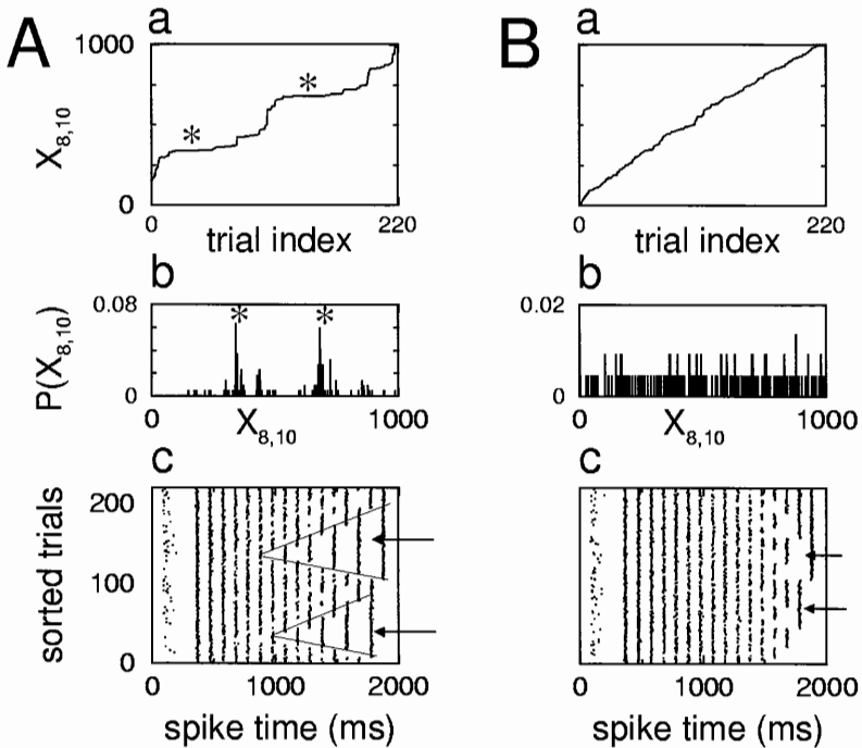
Figure 7: Cortical neuron spike trains had a deterministic structure not present in Poisson-like spike trains. Each trial was assigned a binary representation as described in the text. In A, the original data from Figure 2 and in B spike trains obtained by randomly shuffling spike times of each event across trials were used. In each row, (a) binary representation X_{8,10} , (b) distribution of X_{8,10} values across 220 trials, and (c) rastergram with trials ordered according to value of X_{8,10} , increasing from bottom to top. The stars (*) and the arrows ( \leftarrow ) are described in the text.
