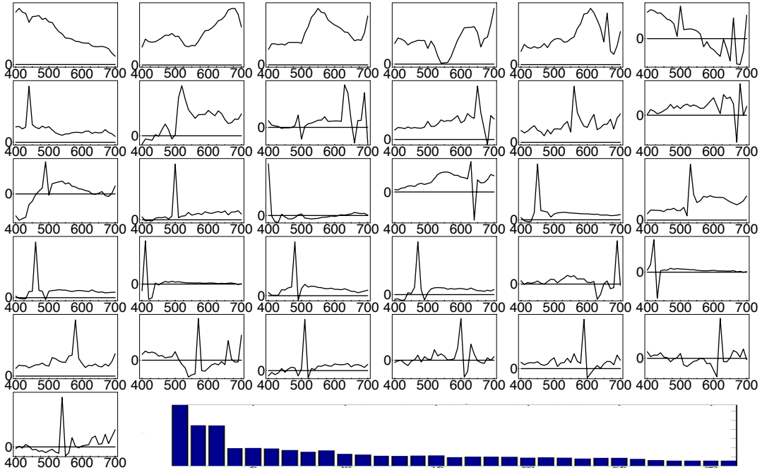
Figure 2: The spectra of the learned basis functions ordered in decreasing L_2 -norm their relative contributions (inset).
